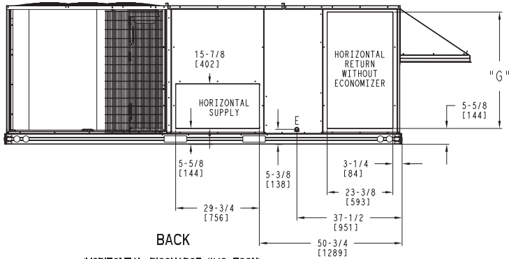
(HORIZONTAL DISCHARGE W/O ECON) (WHEN ORDERED)
