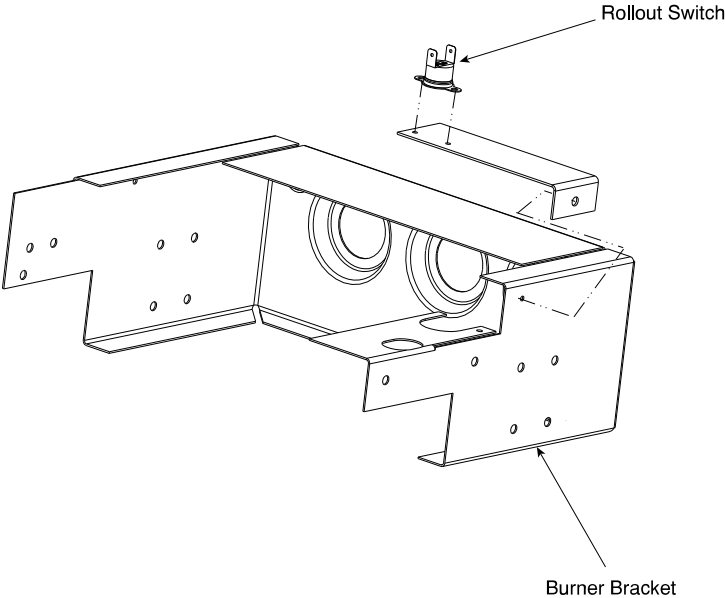
Fig. 9 – Burner Bracket
