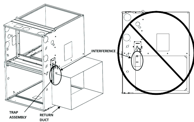
Upflow Right Side Return Configuration - Trap Interference
