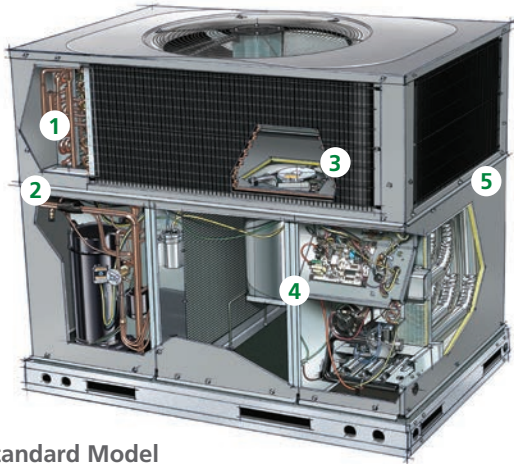
Standard Model
