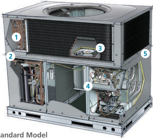
Standard Model
