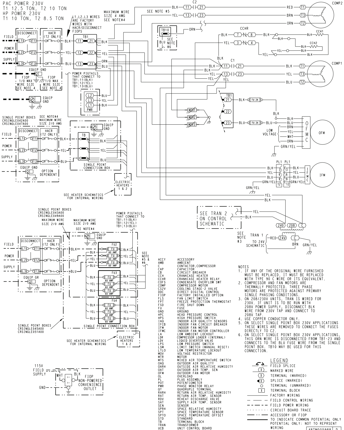
Typical Power Wiring Diagram — RAV150 208-230/3/60 Unit with Electromechanical Controller
