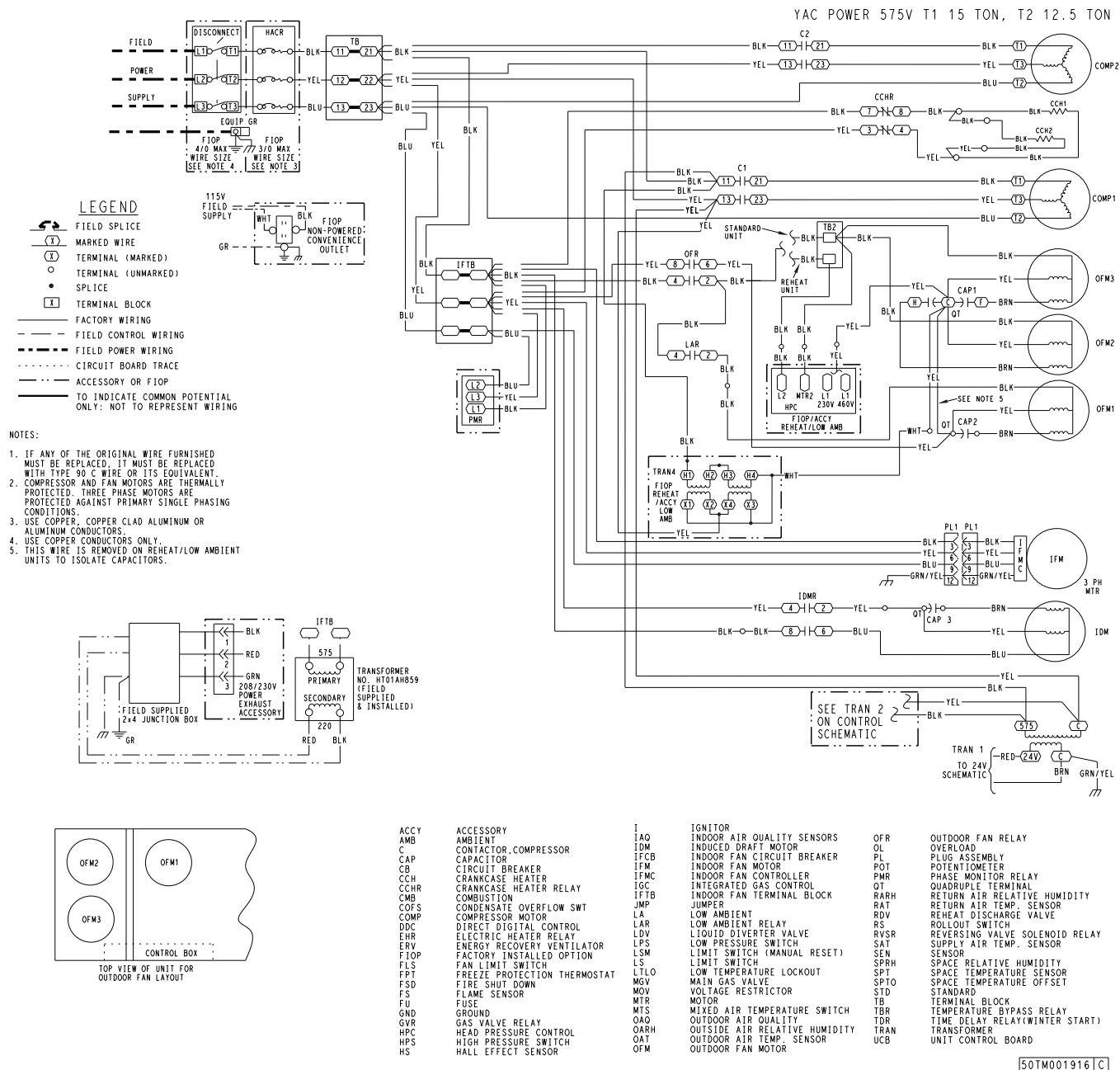
Typical Power Wiring Diagram — RGV180 575-3-60 Unit with Electromechanical Controllers
