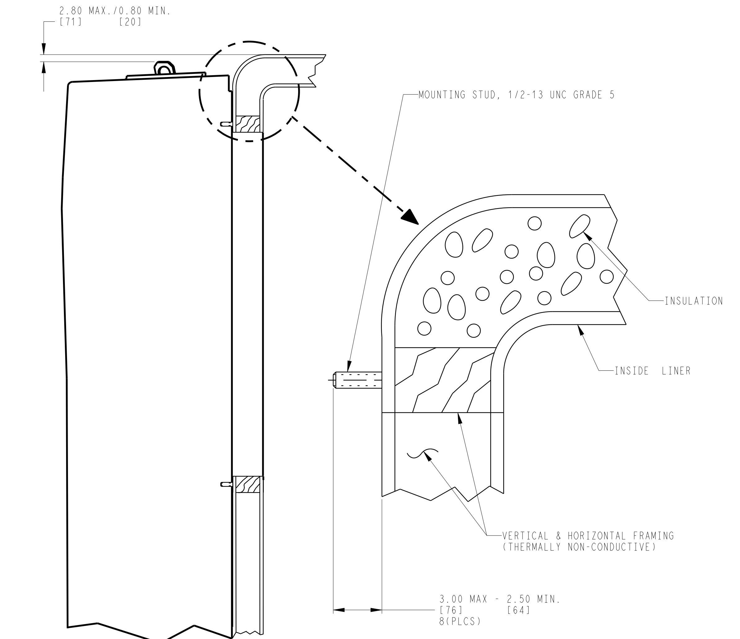
TRAILER SIDE VIEW
