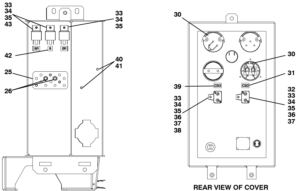
FRONT VIEW WITH COVER REMOVED
