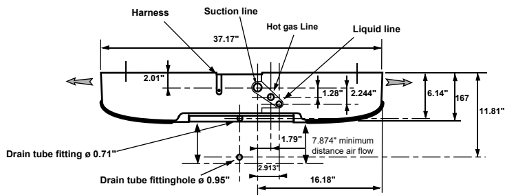
Rear Mounting
