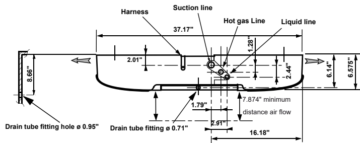
Front and Side Mounting
