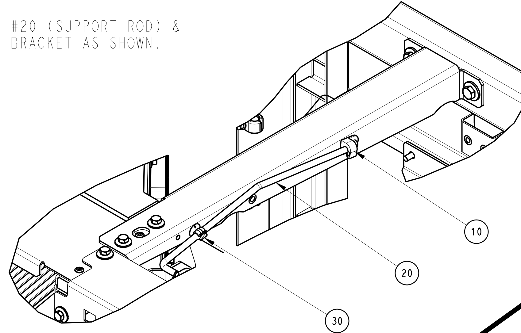
DETAIL A SCALE 0.400
