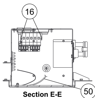
Component Layout
