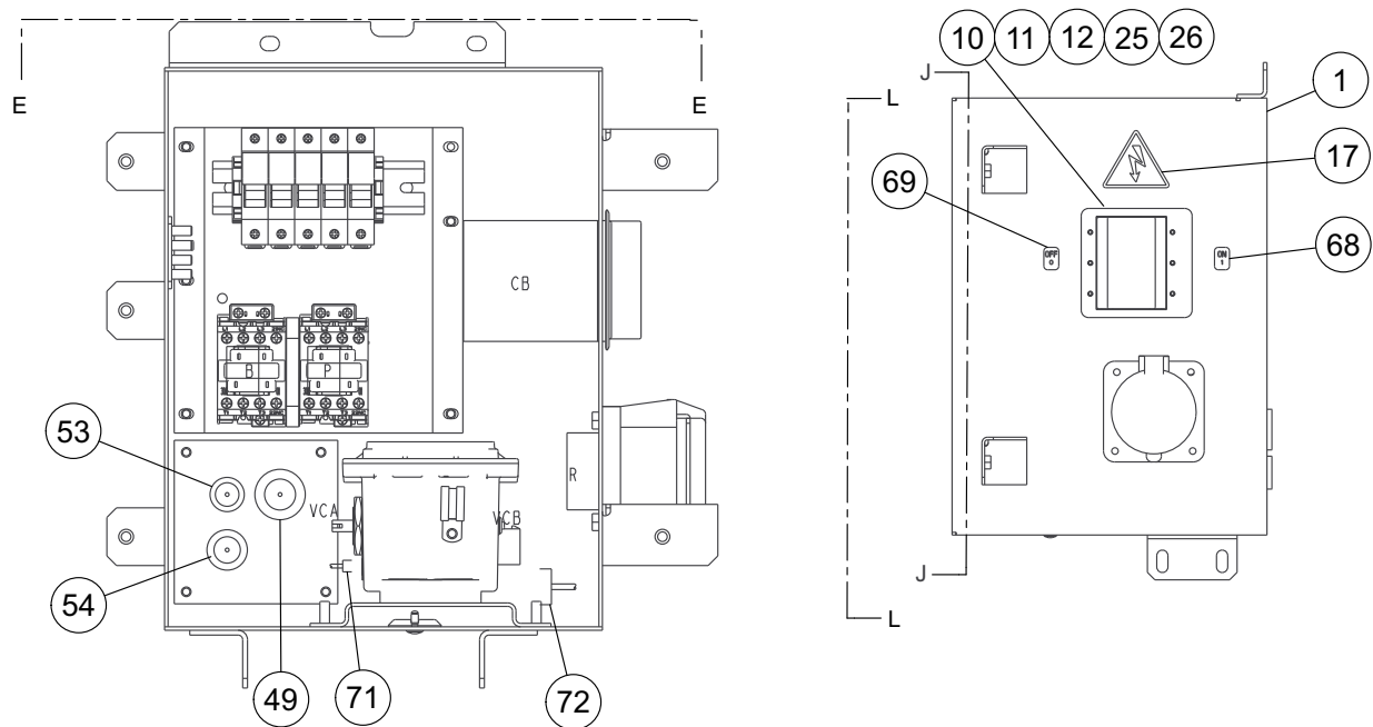
Component Layout
