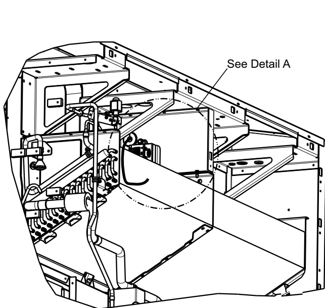
Sensor Location
