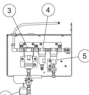
Section C-C H2O Separator / Air Filter
