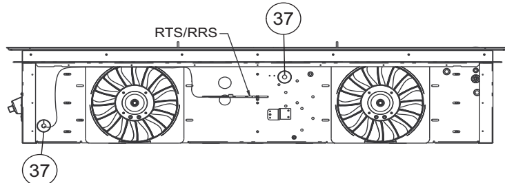
Control Box - Front View
