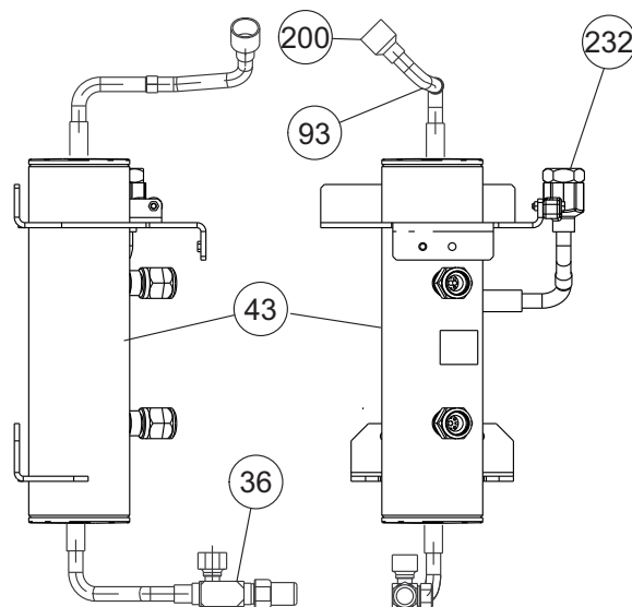
Receiver Brazed Assembly with Pressure Relief Valve
