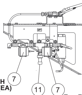
EverFRESH Nitrogen Valve (EN)
