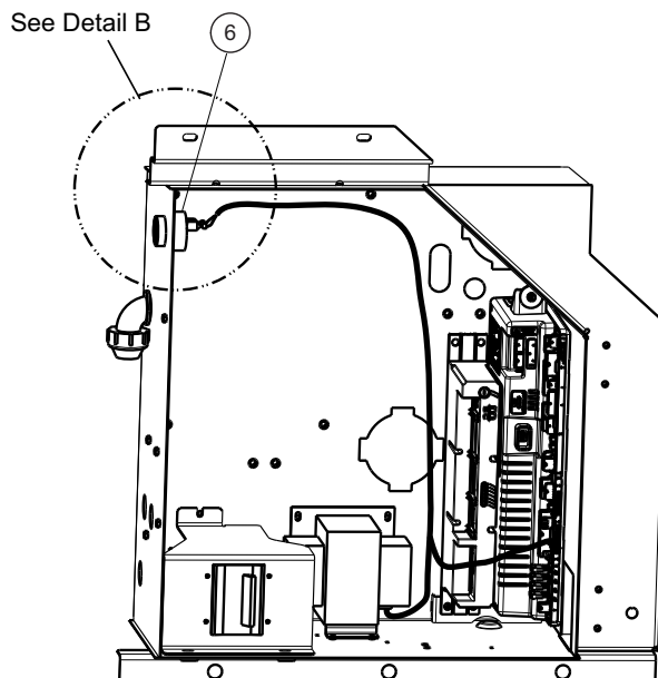
Buzzer Location
