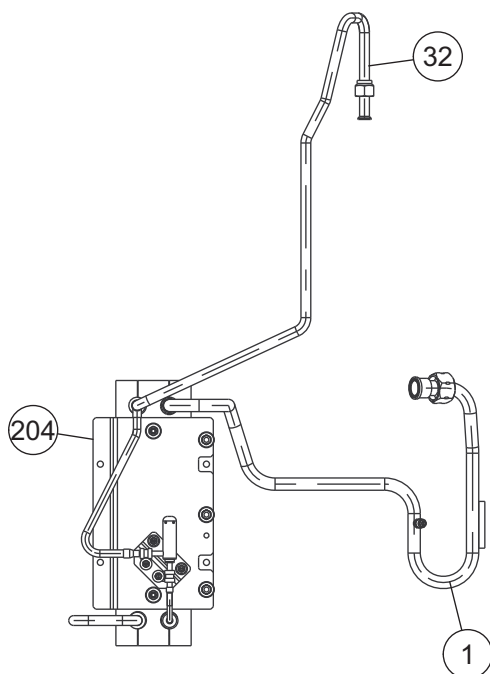
Economizer Brazed Assembly
