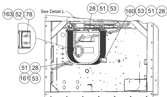
Rear View (Standoff & Fan Deck Assembly)
