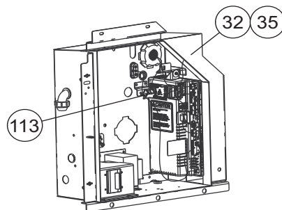
Control Box - Front View
