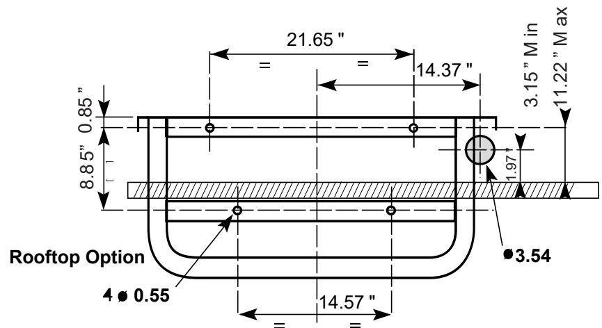
Condenser Installation - Bottom
