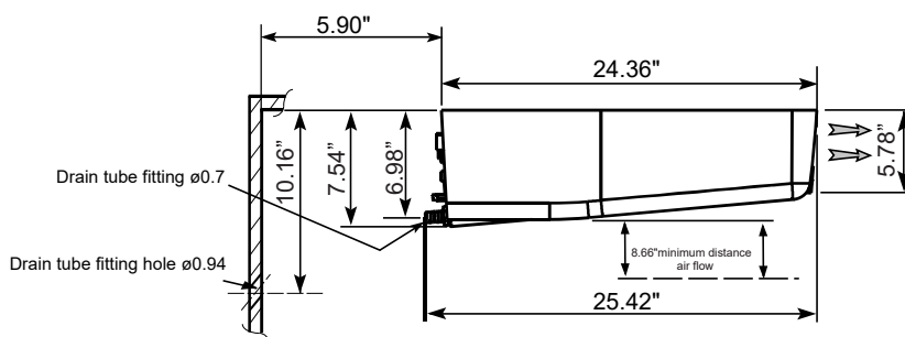
Evaporator Side View
