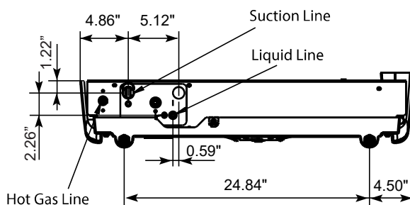
Evaporator Rear View
