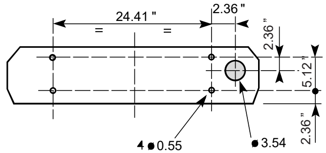
Condenser Installation - Top
