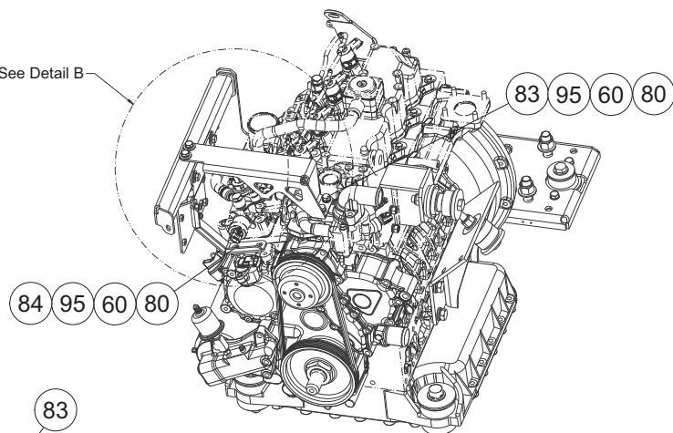
Fan Removed for Clarity
