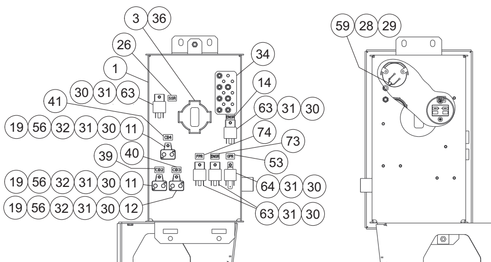
Front View with Cover Removed
