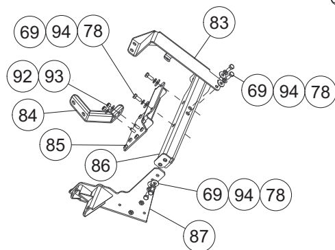
Detail B Radiator / Fuel System Bracket Assy
