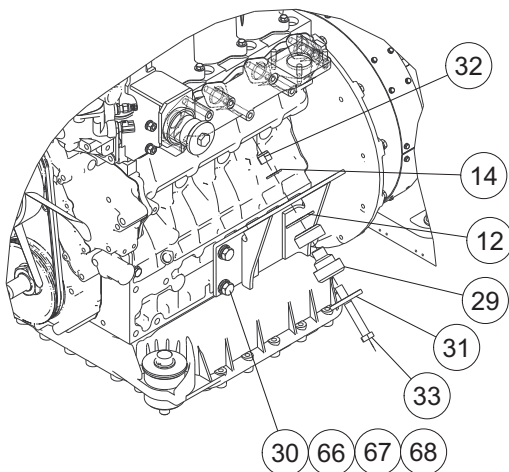
Lower Snubber
