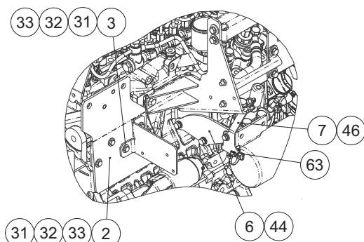
Fuel Filter, Lines, Pump and Air Filter removed for clarity
