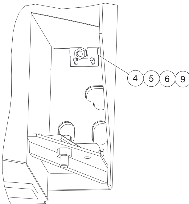
Lower Unit Mtg Area View with Item 11 Removed
