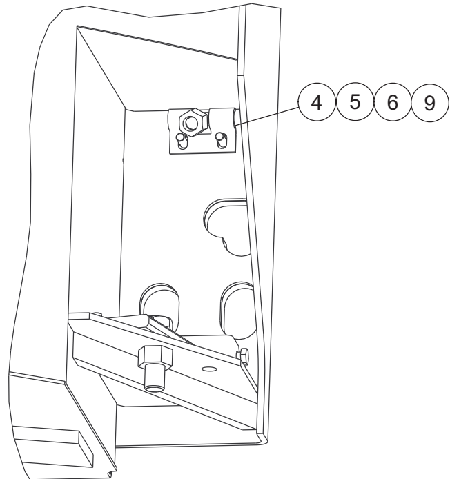
Lower Unit Mtg Area View with Item 11 Removed
