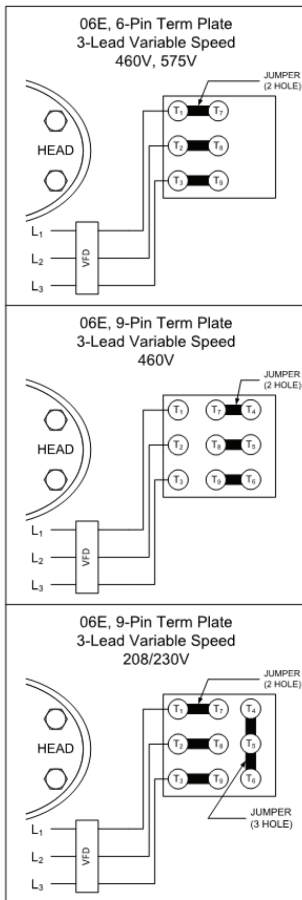
Fig. 18 — 06E Variable Speed Wiring Diagrams
