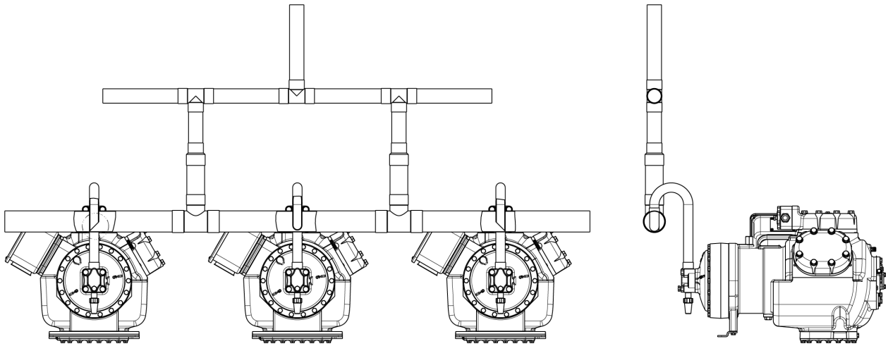
Fig. 5 — Suction Header ABOVE Compressors
