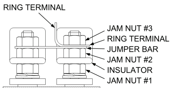
06E TERMINAL PIN WIRING DETAILED VIEW
