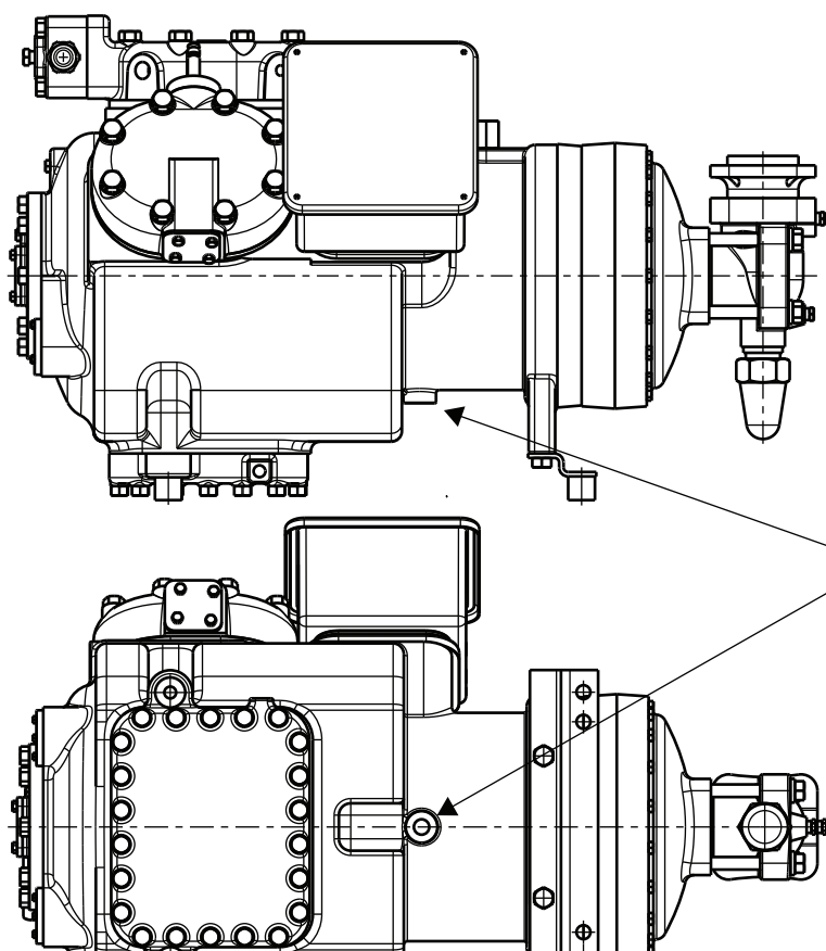
Fig. 11 — 06E Motor Barrel Equalization Port
