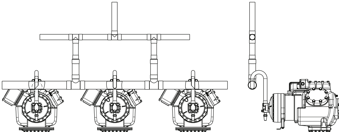
Fig. 5 — Suction Header ABOVE Compressors
