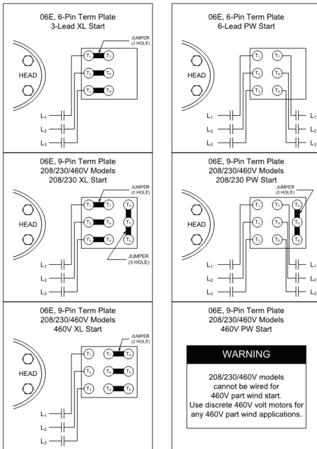
Fig. 16 — 06E Fixed Speed Wiring Diagrams
