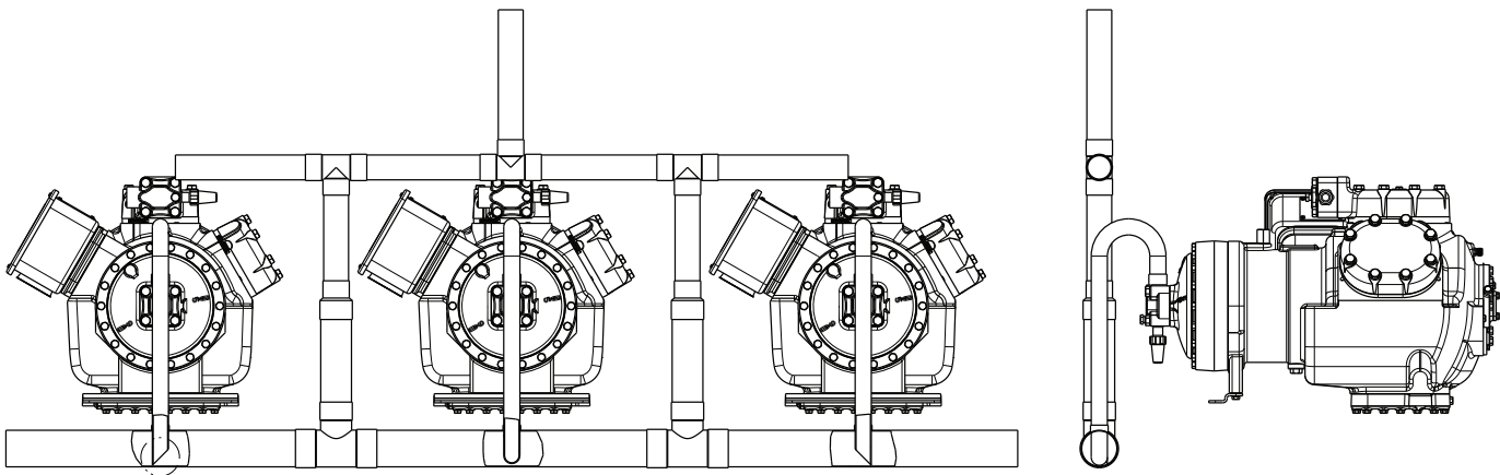
Fig. 4 — Suction Header BELOW Compressors
