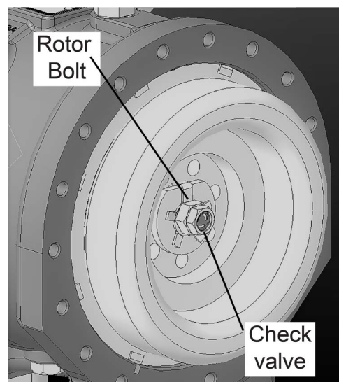
Fig. 10 — Check Valve in 06E Rotor Locking Bolt
