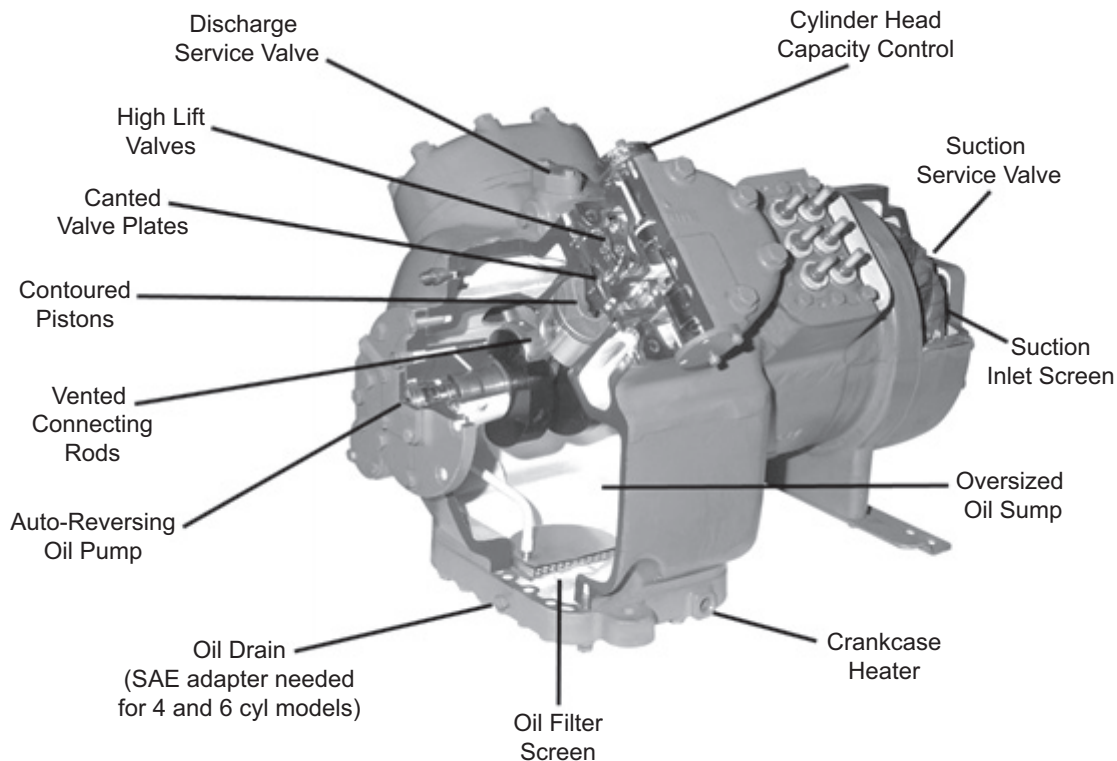
Fig. 1 — Key Features, 06E Semi-Hermetic Reciprocating Compressor
