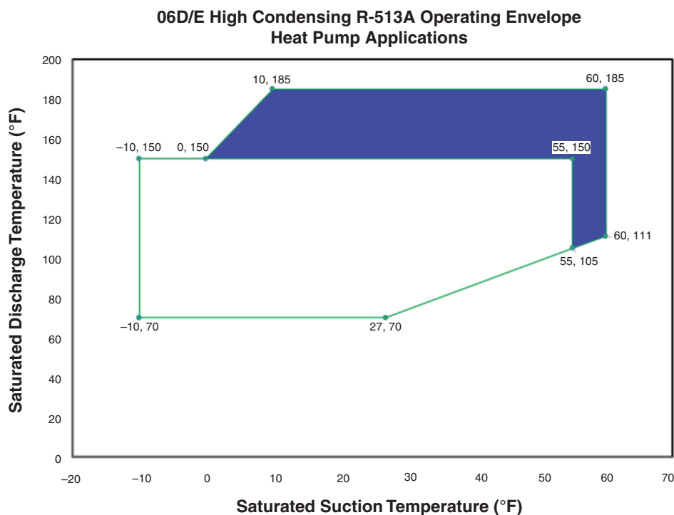
Fig. 19 — 06D/E High Condensing R-513A Operating Envelope Heat Pump Applications
