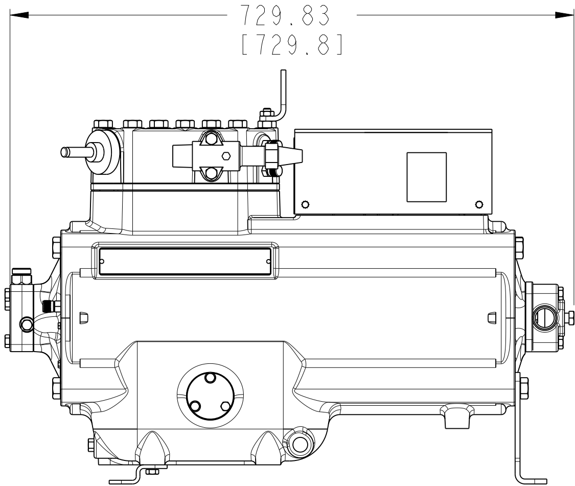
RIGHT VIEW
