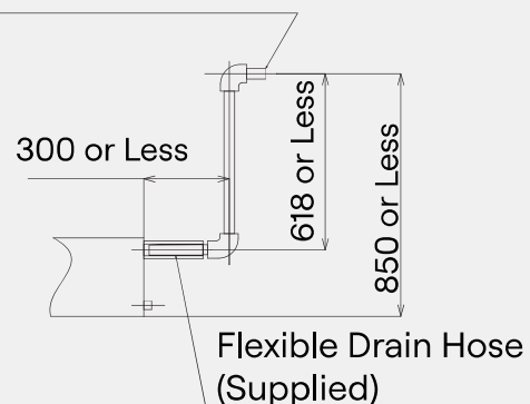
Drain up Setup Dimensions
