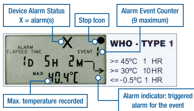
VaxAlert USB in history mode, high alarm event
